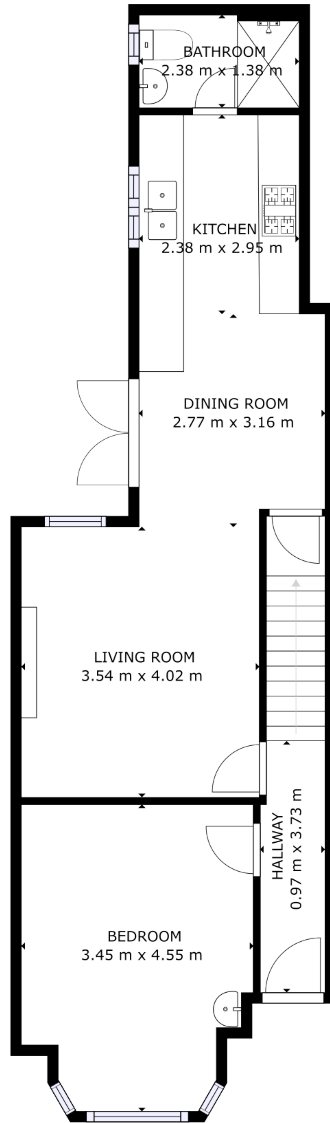
GROUND FLOOR
